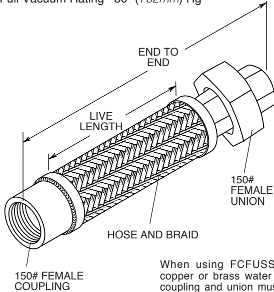
FCFUSS-NSF DIMENSIONS AND PRESSURE RATINGS (American Units)
