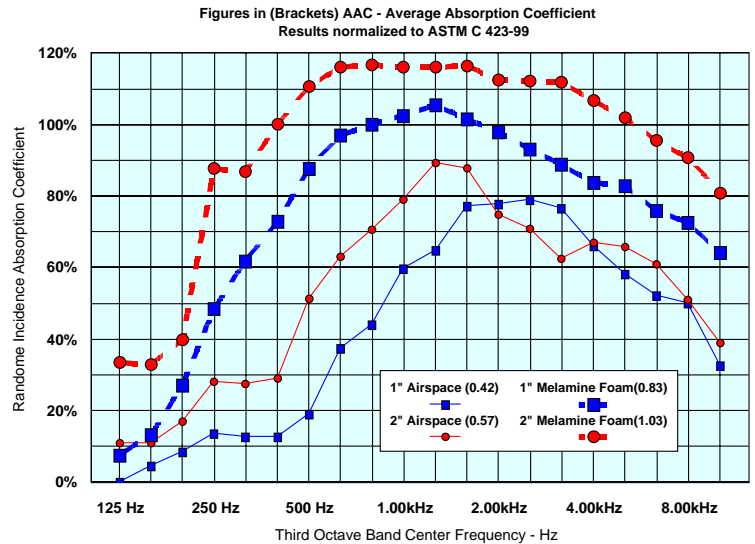
Figure 1 Absorption Factor of 0.040"(1mm) Millennium Metal in a small reverberation chamber.
