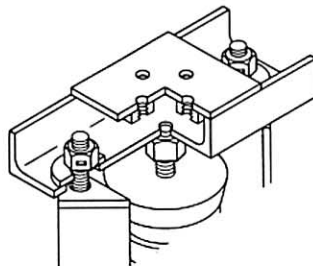
TYPE SLR DIMENSIONS (Inches)
